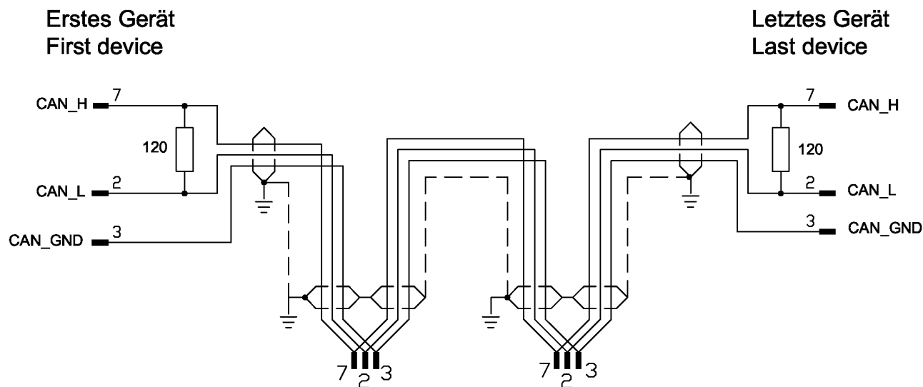
Figure 75: CAN- Network
