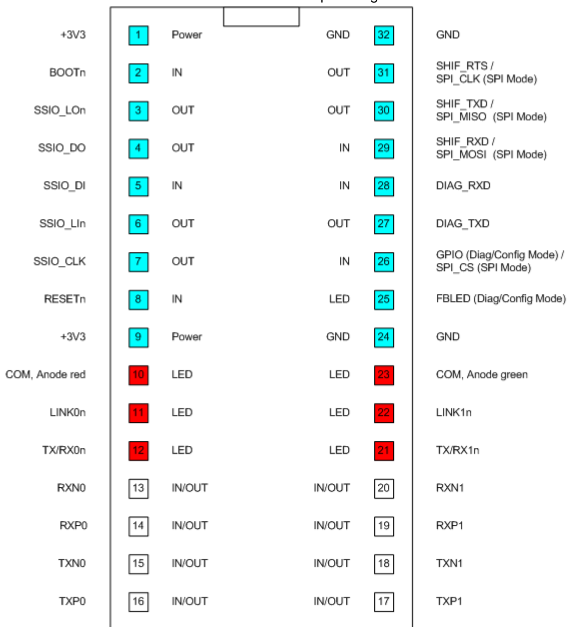
Figure 54: Pinning of NIC 52-RE
