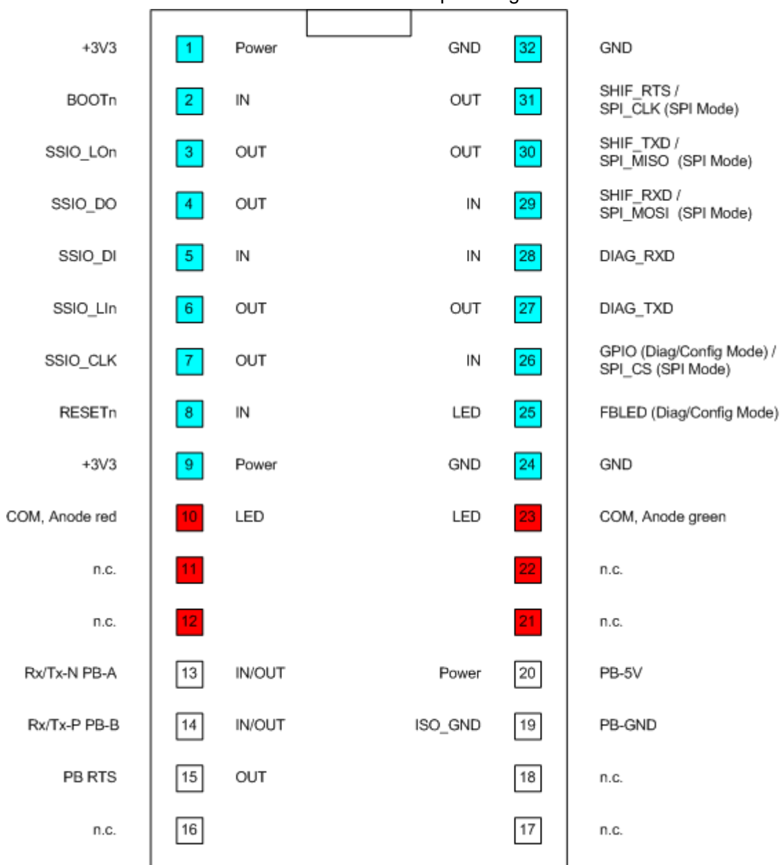
Figure 48: Pinning NIC 50-DPS
