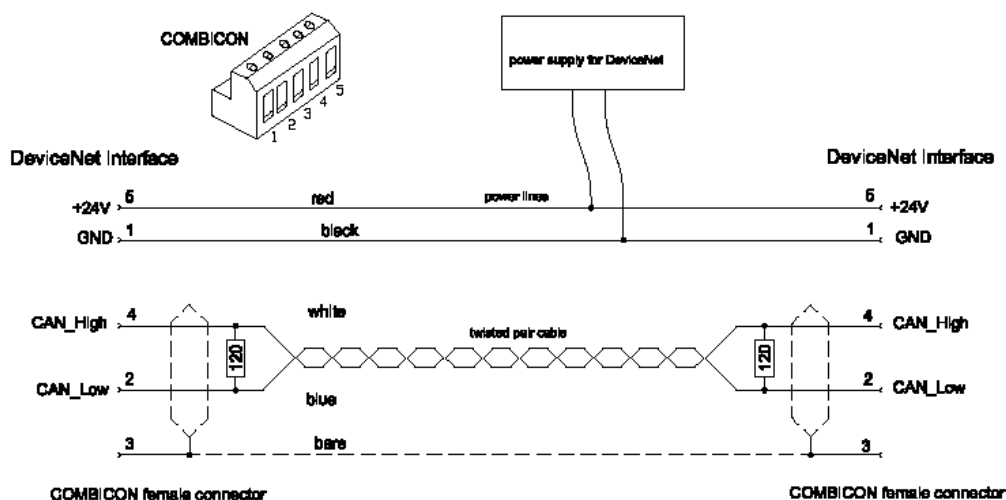
Figure 78: DeviceNet Network
