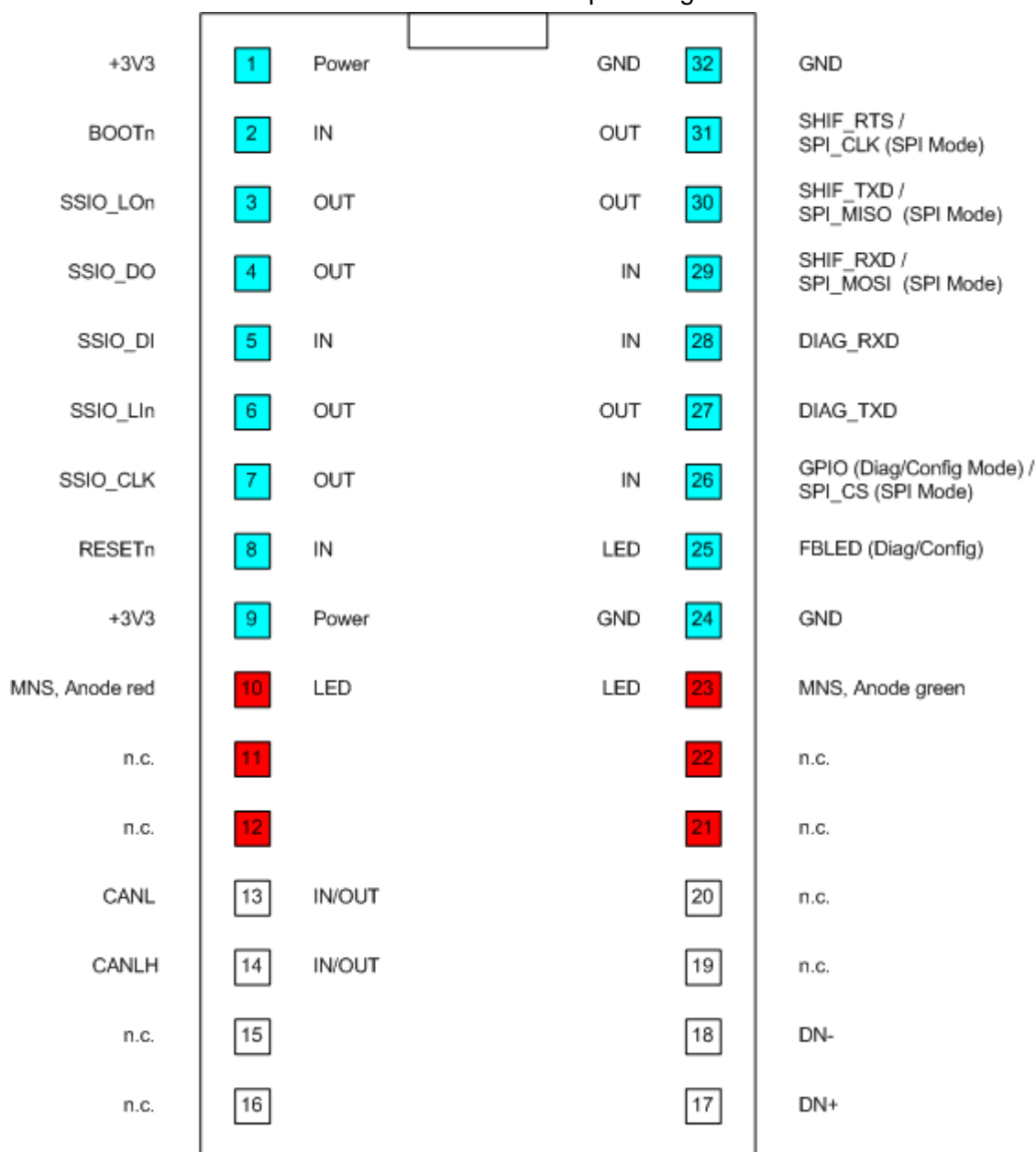
Figure 43: Pinning of NIC 50-DNS
