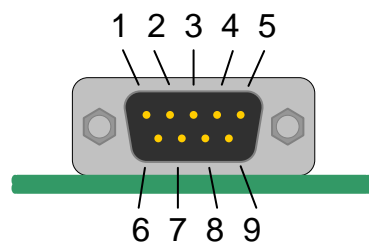
Figure 62: Diagnostic Interface Connector
