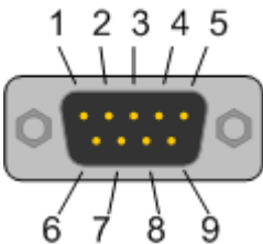
Figure 74: CANopen Interface (DSub male connector, 9 pin) of NICEB-AIF-CO
