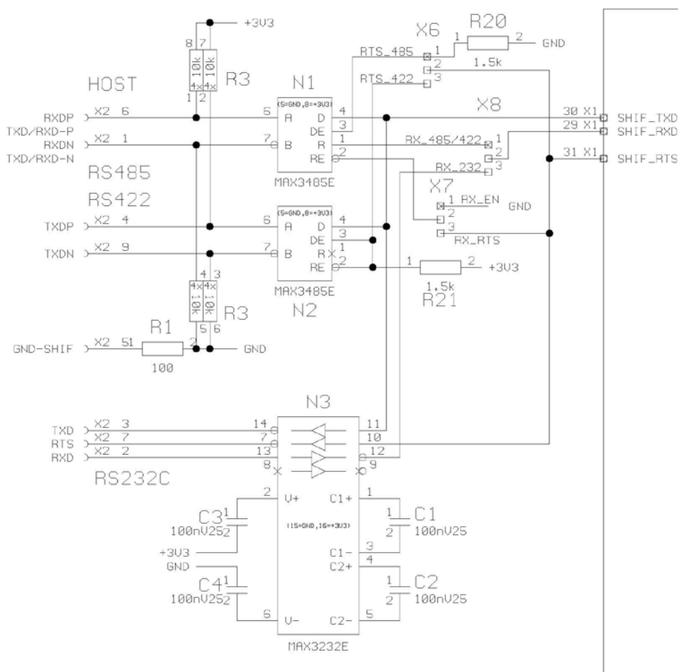
Figure 64: Wiring Diagram of the Serial Host-Interface of the Evaluation Board
