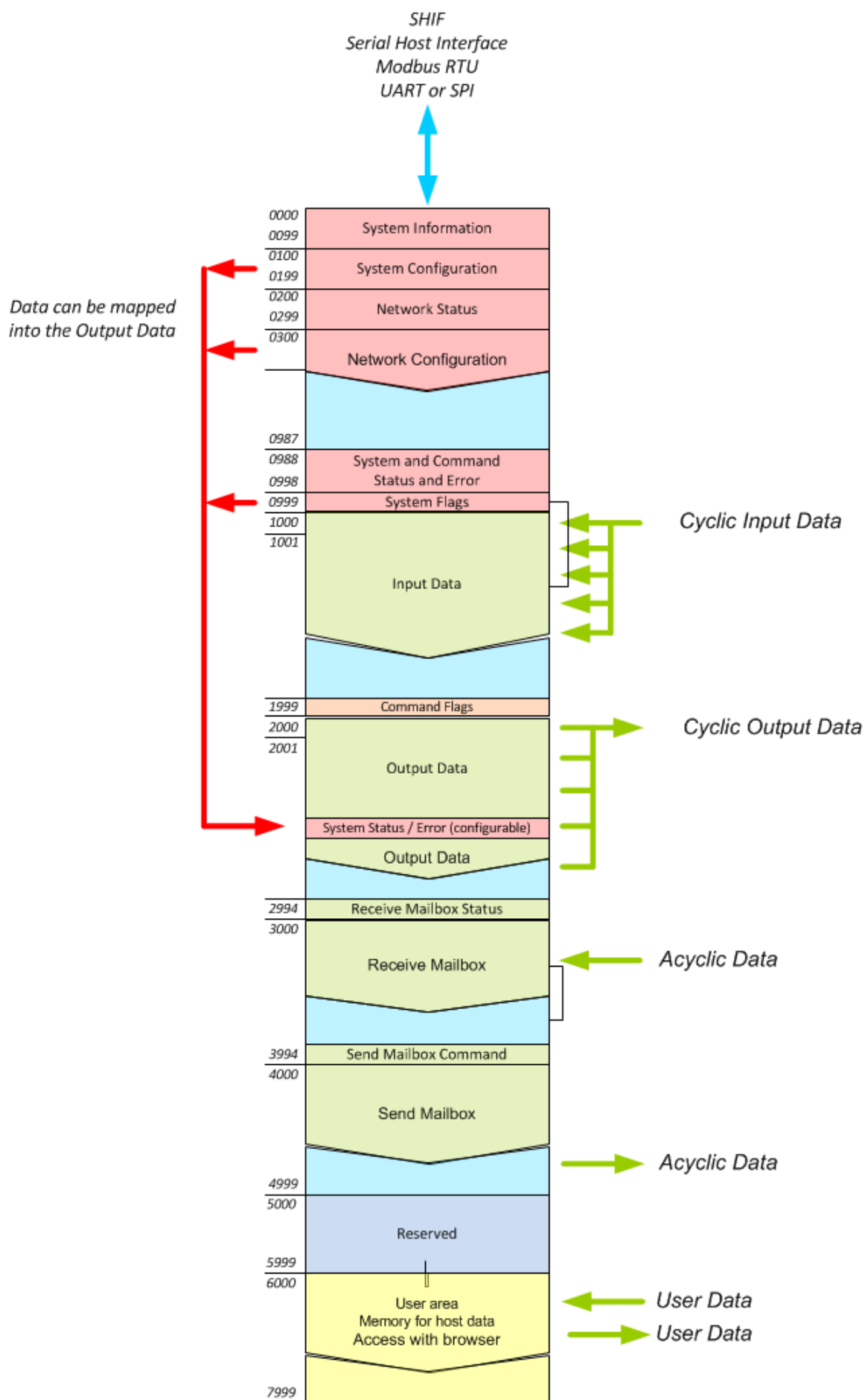
Figure 6: Register Area
